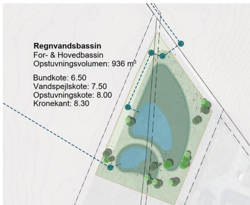
Plan over forsinkelsesbassinet
